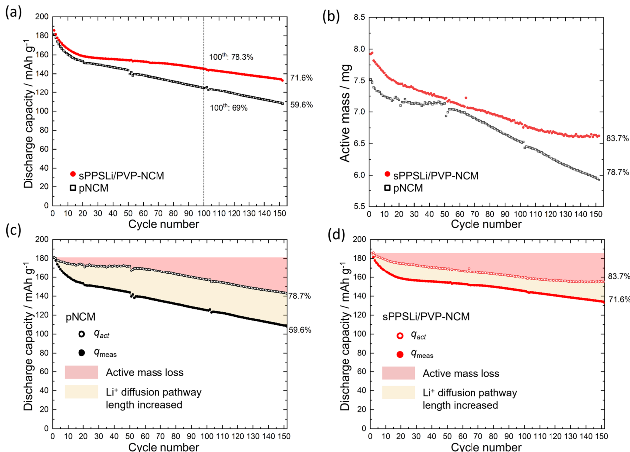
Fig. 4 (a) Cycling performance at 0.1C of \text{LiInSEB/pNCM} and \text{LiInSEB/sPPSLi/PVP-NCM} at 25 °C. (b) Corresponding evolution of m_{\text{act}} . For (c) pNCM and (d) sPPSLi/PVP-NCM, capacity loss is plotted, respectively, and split into the loss of m_{\text{act}} and the loss due to increased \text{Li}^+ diffusion pathway length. The pink area represents the loss of m_{\text{act}} . The yellow area illustrates the increasing \text{Li}^+ diffusion pathway length, determined as the difference between q_{\text{meas}} and q_{\text{act}} .
