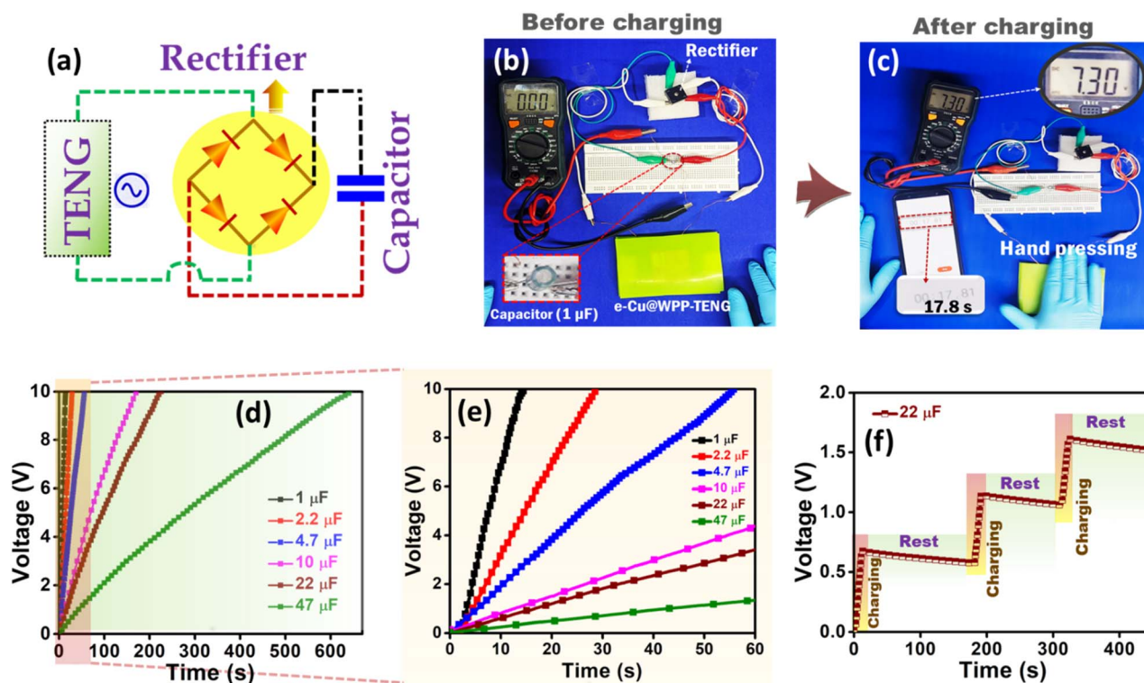
Fig. 5 (a) Circuit diagram for charging the capacitor by using e-Cu@WPP-TENG, (b) & (c) digital photographs showing the 1 \mu\text{F} capacitor before and after charging by using e-Cu@WPP-TENG, (d) voltage–time plot showing the charging of different capacitors by using e-Cu@WPP-TENG, (e) zoomed-in portion of (d) showing the charging of capacitors in a 1 minute time period, and (f) voltage–time plot for a 22 \mu\text{F} capacitor with alternating charging and rest periods provided by hand pressing of e-Cu@WPP-TENG.
