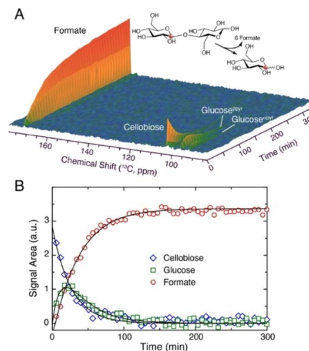
Fig. 6 Real-time observation of the conversion. Reaction conditions: 0.05 M [1'-^{13}\text{C}] cellobiose, 0.6 M LiOH and 24 equiv. hydrogen peroxide in a 3 mm NMR tube (200 \mu\text{L} \text{H}_2\text{O}/\text{D}_2\text{O} (90%/10%)) at 308 K without agitation.
