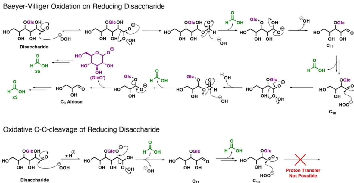
Scheme 3 Plausible mechanisms in the degradation of cellobiose in the presence of a hydroperoxyl anion. The absence of C10 disaccharide and the rapid and full conversion to formate argue for a central role of Baeyer–Villiger oxidation.
