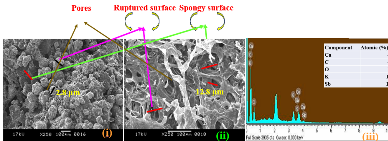
Fig. 10 (a). Effect of CHNSO composition on pyrolysis char; (b) (i) SEM micrograph of orange peel waste; (ii) SEM micrograph of pyrolyzed orange peel waste; (iii) EDX spectrum of pyrolyzed orange peel waste.
