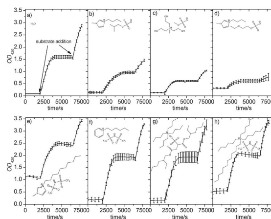
Fig. 8 Time course of laccase-catalysed ABTS oxidation in the presence of ILs. 96 (a) Control. (b) [C_4\text{mim}][C_3(2-C_1)OSO_3] , (c) [N_{1,2}(\text{OH})_3][C_1OSO_3] , (d) [C_4\text{mim}][C_2OC_2OSO_3] , (e) [C_{10}\text{mim}][\text{NTf}_2] , (f) [C_6\text{py}][\text{NTf}_2] , (g) [N_{4,4,4,4}][\text{AOT}] , and (h) [\text{P}_{6,6,6,14}][\text{NTf}_2] . (b), (c), and (d) are aqueous buffer (pH 4.5) solutions of the water-miscible ILs (20% (v/v)). (e), (f), and (g) are biphasic mixtures of buffer (pH 4.5) with water-immiscible ILs (20% (v/v)). Copyright RSC, 2012.
