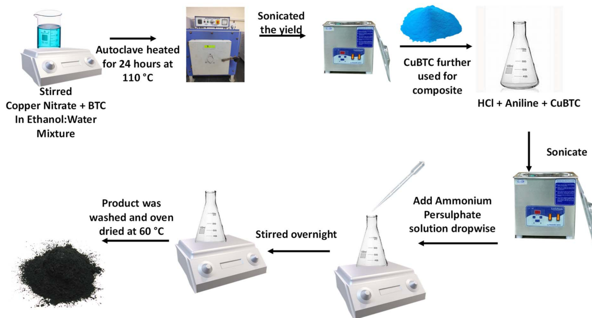
Scheme 1 Synthesis of the PANI/CuBTC photocatalyst.
