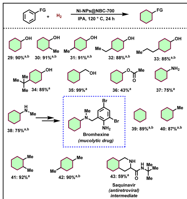
Scheme 2 Ni-NPs@NBC-700 catalyzed ring hydrogenation of functionalized arenes. a Reaction conditions: 0.5 mmol substrate, 50 mg catalyst, 50 bar \text{H}_2 , 2 mL isopropanol, 120 °C, and 24 h; isolated yield. b GC yields using n -hexane as the standard.
