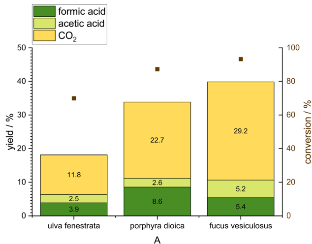
Fig. 5 Screening of different macroalgae in the OxA process for their product yield (left y-axis) and algae conversion (right y-axis) using the HPA-2 catalyst. Reaction conditions: HPA-2 at an initial temperature of 90 °C, non-isothermal reaction, 30 bar oxygen pressure, 1000 rpm stirrer speed, 24 h reaction time. The liquid phase consisted of 200 g of water with 10 g suspended macroalgae and 1.95 g of dissolved catalyst (1 mmol, HPA-2).
