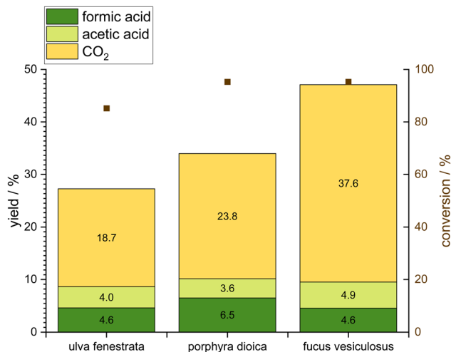
Fig. 4 Screening of different macroalgae in the OxA process for their product yield (left y-axis) and algae conversion (right y-axis) using the HPA-5 catalyst. Reaction conditions: HPA-5 at an initial temperature of 90 °C, non-isothermal reaction, 30 bar oxygen pressure, 1000 rpm stirrer speed, 24 h reaction time. The liquid phase consisted of 200 g of water with 10 g of suspended macroalgae and 1.89 g of dissolved catalyst (1 mmol, HPA-5).
