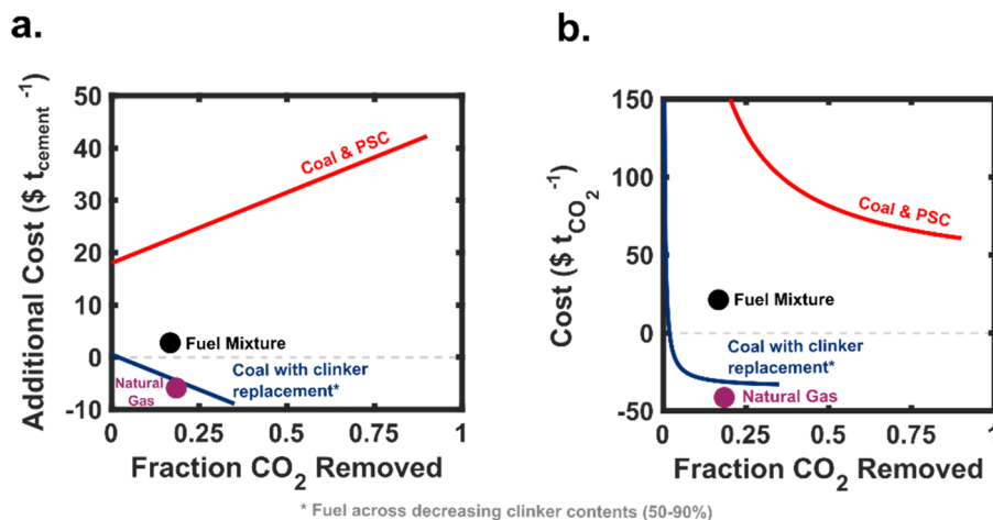
Fig. 2 (a) Additional costs of implementing the decarbonization technology for cement production ( \$ t_{cement}^{-1} ) beyond the current baseline costs of cement production ( \$106 t_{cement}^{-1} ). (b) Costs of CO_2 removal ( \$ t_{CO_2}^{-1} ) associated with pursuing clinker replacement, fuel replacement, and/or retrofitting a capture unit onto the plant with varying costs of capture. The costs of capture at the maximum capture fraction of 90% are \$60 t_{CO_2}^{-1} , in line with current PSC systems. The fuel alternatives are single data points because the technology can only remove a set amount of CO_2 when the fuel is replaced. On the contrary, the clinker replacement and PSC curves represent the range of decarbonization amounts that can result by varying the amount of clinker replaced or CO_2 captured, respectively. The dashed gray line at $0 in both figures represents the baseline costs.
