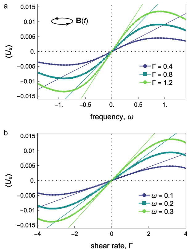
Fig. 4 Rotating field. Time-averaged particle velocity in the x -direction, perpendicular to flow, as a function of (a) frequency \omega and (b) shear rate \dot{\Gamma} . Markers show numerical integration results; solid lines show the approximation of eqn (19), valid at low \omega and \dot{\Gamma} . All quantities are made dimensionless using the characteristic scales of eqn (5).
