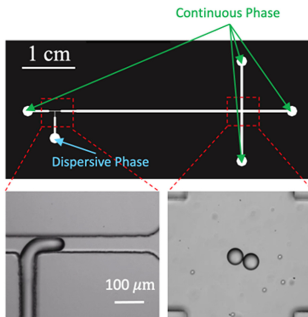
Fig. 3 (Top) A microfluidic Stokes trap device is used for coalescence experiments. The height of the channel is 120 μm, and the channel width at the cross-slot is 400 μm. One liquid is injected into the 4 ports as a continuous phase and another liquid is injected as the dispersive phase. (Bottom Left) The droplets are generated at the T-junction. (Bottom Right) Droplets are trapped at the stagnation point of the cross-slot and interact with the following droplets. Note that the bottom images are of only a sub-portion of the region indicated by the red dashed boxes.
