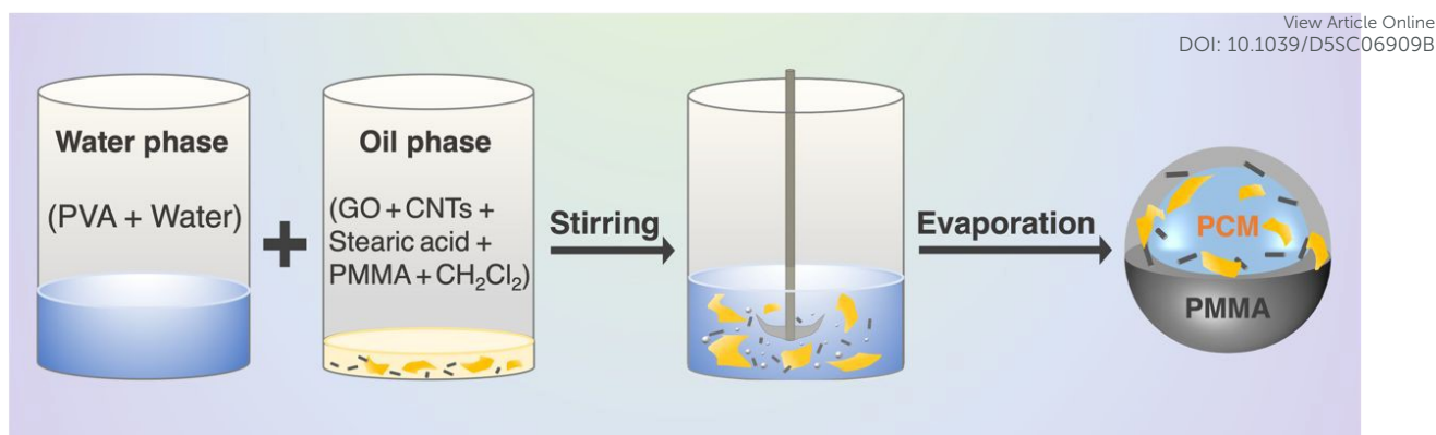
Scheme 1. Schematic illustration of the synthesis of the PCM-GO/CNTs microcapsules.
