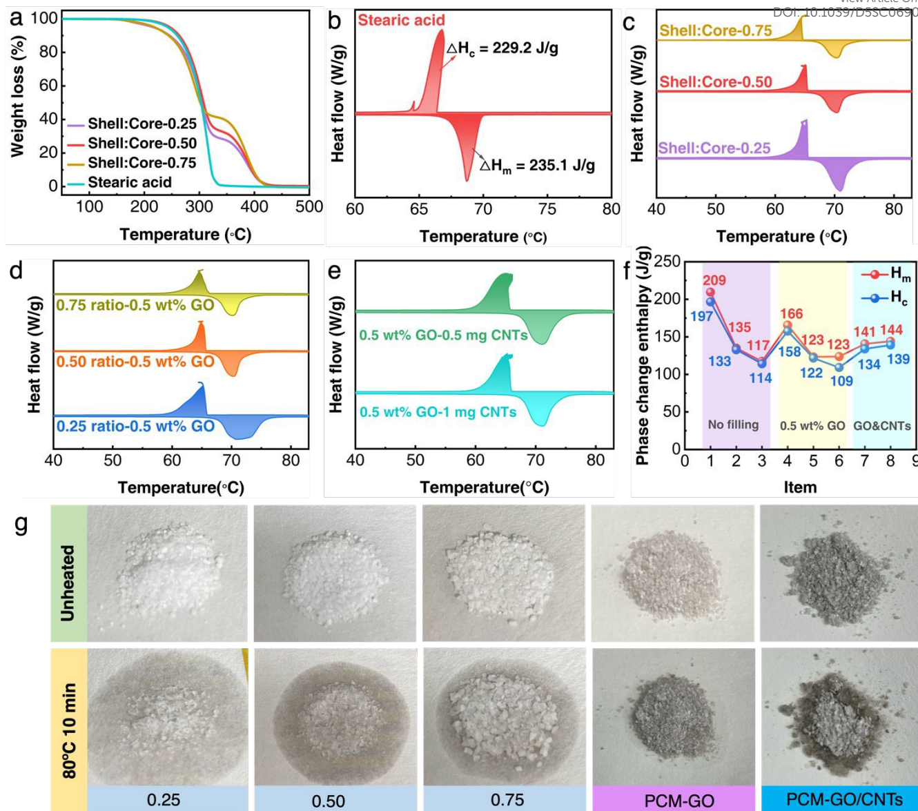
Figure 4. (a) TGA , and DSC curves comparing (b) pure stearic acid with (c) PCMs microcapsules of different shell/core ratios. (d) different shell/core ratio with 0.5 wt% GO, and (e) 0.5 mg and 1.0 mg CNTs of PCMs-GO (0.5 wt%) microcapsules. (f) Phase change enthalpies of PCMs microcapsules with different high-conductivity materials, including (1) different shell/core ratio (0.25, 0.50, and 0.75) without filling; (2) different shell/core ratio (0.25, 0.50, and 0.75) with 0.5 wt% GO; (3) Same shell/core ratio (0.50) and 0.5 wt% GO filling with 0.5 mg and 1.0 mg CNTs. (g) Leakage tests of diferent ratio (0.25, 0.50, 0.75) of PCM microcapsule, PCM-GO microcapsules and PCM-GO/CNTs microcapsules
