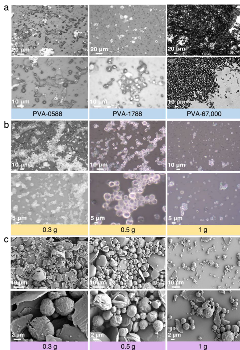
Figure 1. Optical images of PCMs microcapsules with different (a) emulsifier types, and (b) content of PVA-67,000. (c) SEM images of PCM microcapsules with different content of PVA-67,000.
