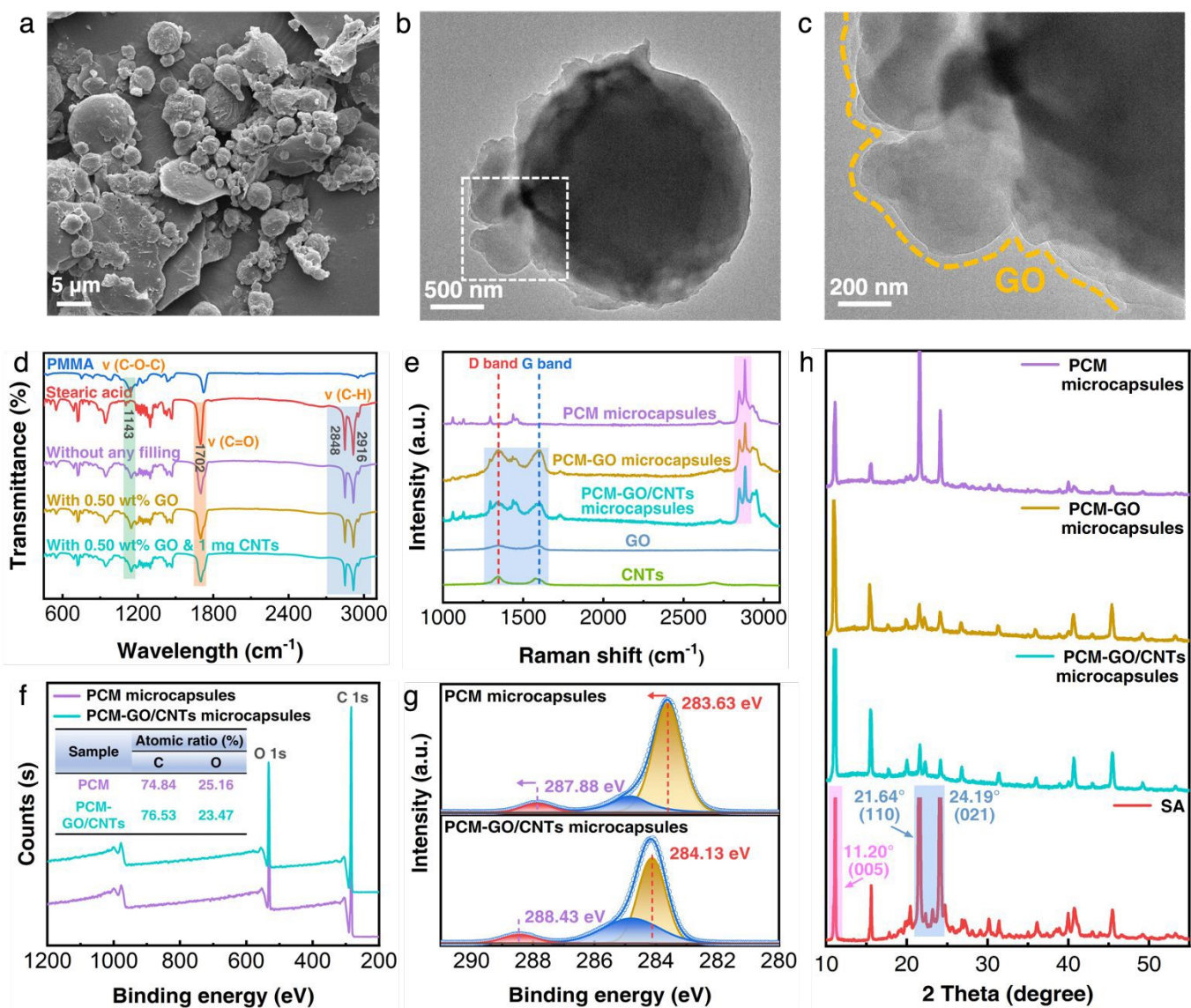
Figure 3. (a) SEM, (b) and (c) TEM images of PCM-GO/CNTs microcapsules. (d) FTIR spectra of (1) pure PMMA , (2) pure stearic acid, (3) 0.50 shell/core ratio of PCMs microcapsules , (4) 0.50 shell/core ratio with 0.5 wt% GO, and (5) 1.0 mg CNTs of PCMs-GO (0.5 wt%) microcapsules. (e) Raman scattering spectra of the PCM microcapsules, PCMs-GO microcapsules, PCMs-GO/CNTs microcapsules, GO and CNTs. (f) XPS spectra and (g) high-resolution C 1s spectra of PCM microcapsules and PCM-GO/CNTs microcapsules. (h) XRD patterns of (1) 0.50 shell/core ratio of PCMs microcapsules , (2) 0.50 shell/core ratio with 0.5 wt% GO, (3) 1.0 mg CNTs of PCMs-GO (0.5 wt%) microcapsules and (4) pure stearic acid.
