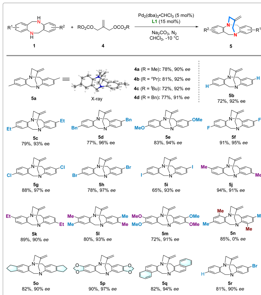
Fig. 3 Substrate scope of propeno -TBs. Unless otherwise indicated, the reaction conditions were as follows: 1 (0.1 mmol, 1 equiv.), 4 (0.15 mmol, 1.5 equiv.), \text{Pd}_2(\text{dba})_3 \cdot \text{CHCl}_3 (5 mol%), L1 (15 mol%), and \text{Na}_2\text{CO}_3 (0.2 mmol, 2 equiv.) in \text{CHCl}_3 (1 mL) under a \text{N}_2 atmosphere at -10^\circ\text{C} for 18 h.
