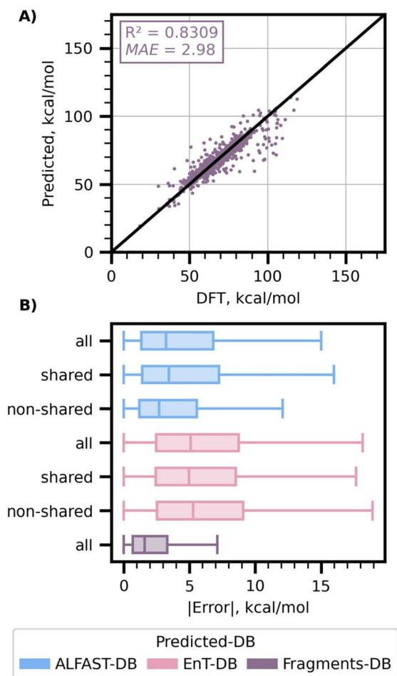
Fig. 7 (A) Predicted vs. computed S_0 - T_1 adiabatic gaps of the model trained on the Fragments-DB. (B) Boxplots with total (all) and marginal absolute error distributions of molecules based on whether they have a shared fragment in Fragments-DB (shared vs. non-shared).
