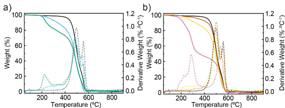
Fig. 2 (a) TGA analysis (air, 10 °C min -1 ) of (6,5)-SWNT (black), eW \rhd SWNT (green), and the mixture of 1 and 2 with (6,5)-SWNTs in the absence of cat. TFA (blue). (b) TGA analysis (air, 10 °C min -1 ) of (6,5)-SWNT (black), the supramolecular complexes formed by the combination of (6,5)-SWNTs and 1 (yellow) or 2 (orange) and the equimolar mixture of 1 and 2 in absence of (6,5)-SWNTs (pink).
