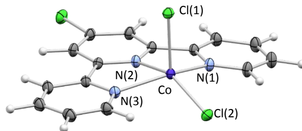
Figure 1. Experimental SC-XRD structure of 1 at 20 K (90% probability ellipsoids). Atom colours: Co (dark blue), Cl (green), N (light blue), C (grey) and H (white). Complex 2 is isostructural to 1 but has two bromide ions bound to Co instead of two chloride ions.
