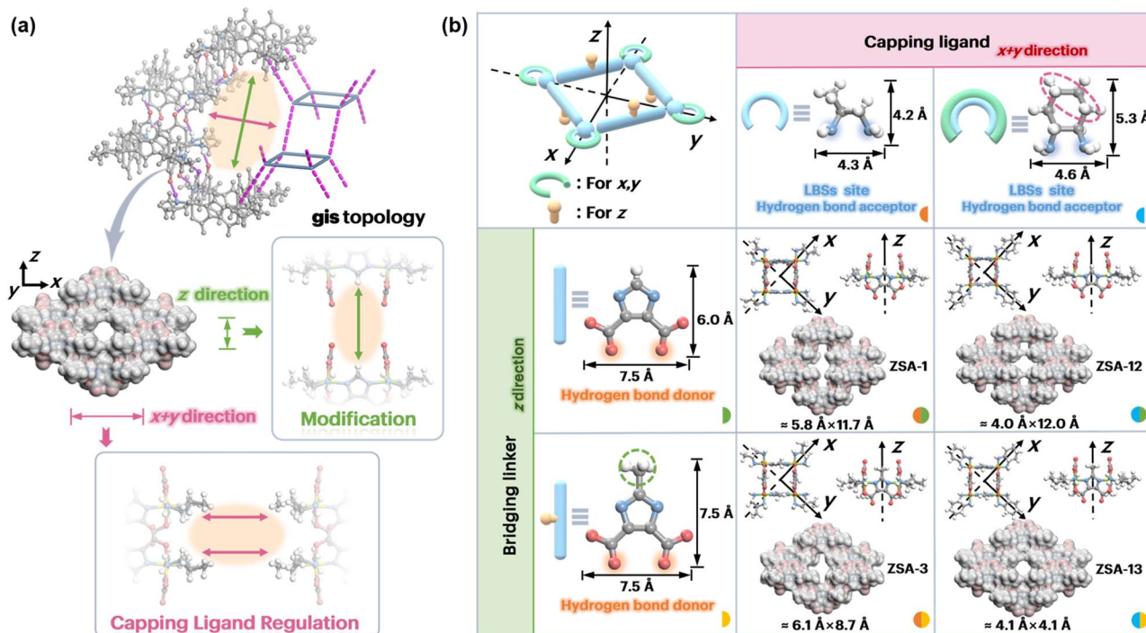
Fig. 1 (a) Schematic illustration of the hydrogen-bonding, topology, and pore regulation in ZSAs; (b) x, y, and z axes in the MOS, showing the dimensions of the bridging and capping ligand and the pore sizes in the ZSAs.
