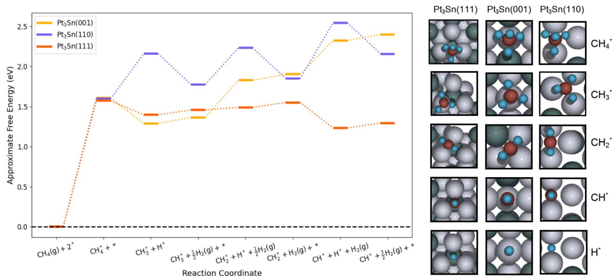
Fig. 7 Reaction profile of the dehydrogenation of methane on \text{Pt}_3\text{Sn}(111) , \text{Pt}_3\text{Sn}(001) , and \text{Pt}_3\text{Sn}(110) at 1 barr and 900 K. Visualizations of the global minimum structures are given on the right hand side. Asterisks above adsorbates indicate a bound species, asterisks on their own denote a bare slab.
