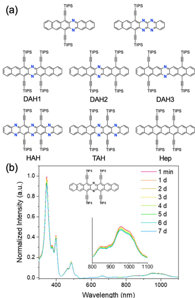
Fig. 43 (a) Representative nitrogen-doped higher acenes with TIPSethynyl groups. The heptacene derivative (Hep) is also shown as a reference. (b) Time-dependent evolution of UV-vis absorption spectra of DAH1 ( 10^{-5} \text{ mol L}^{-1} in dry \text{CH}_2\text{Cl}_2 ) under ambient light and atmospheric conditions. Adapted with permission from ref. 172. Copyrights 2024 American Chemical Society.
