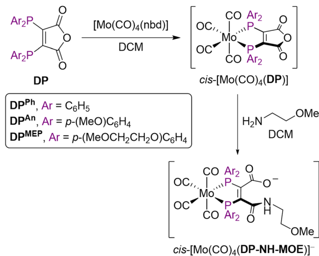
Scheme 2 Mo(0) complexation of DP ligands to give \text{cis-}[\text{Mo}(\text{CO})_4(\text{DP})] and subsequent ring-opening to give \text{cis-}[\text{Mo}(\text{CO})_4(\text{DP-NH-MOE})]^- .
