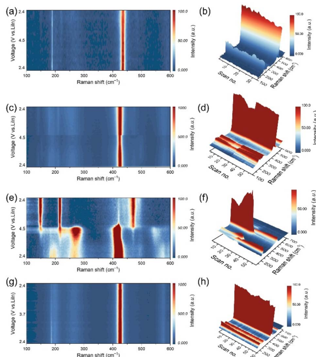
Fig. 2 The in situ Raman spectra of (a and b) LPSCI-VGCF|LPSCI|LiIn, (c and d) uncoated LNMO-LPSCI-VGCF|LPSCI|LiIn, (e and f) LTA@LNMO-LPSCI-VGCF|LPSCI|LiIn, and (g and h) LCO-LPSCI-VGCF|LPSCI|LiIn cells from two-dimensional and three-dimensional views, respectively. The positions for Raman signal collection are the LPSCI-rich area far from the cathode active particle/LPSCI particle interface in the composite cathode.
