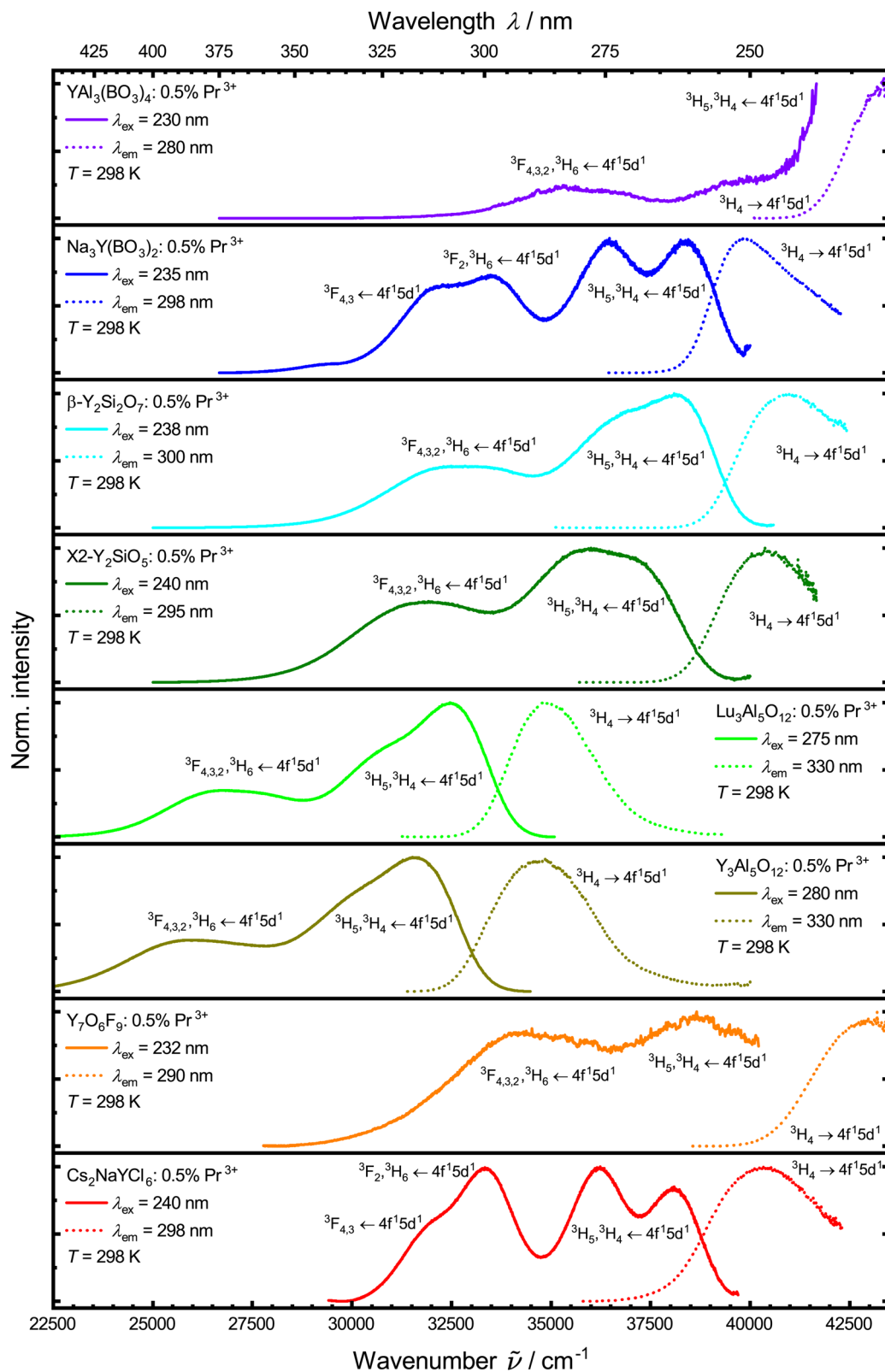
Fig. 5 Normalized photoluminescence emission (solid lines) and excitation spectra (dotted lines) of the synthesized samples at 298 K in UV range showing emission and excitation of 4\text{f}^15\text{d}^1 states. Spectra were measured against wavelengths and converted to wavenumbers using a Jacobian transformation. 99
