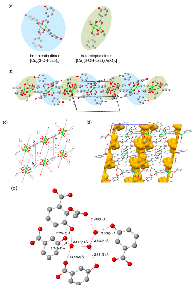
Fig. 1 Crystal structure of 1·3H 2 O. (a) Two types of contributing paddlewheel dimers forming (b) a 1D zigzag chain structure. (c) Packing of the chains, (d) one-dimensional channel structure, and (e) hydrogen bonds involving guest water molecules. The green, blue, gray, and red represent copper, nitrogen, carbon, and oxygen, respectively. Hydrogen atoms are omitted for clarity except in (d). Red dashed lines represent hydrogen bonds.
