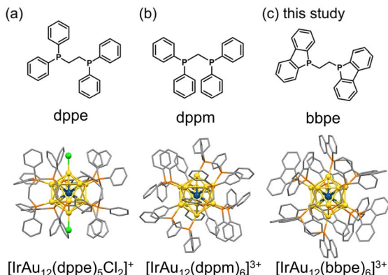
Fig. 1 The molecular structures of the diphosphine ligands and the corresponding Ir@Au 12 clusters for (a) [IrAu 12 (dppe) 5 Cl] + ( IrAu 12 -e-Cl ), (b) [IrAu 12 (dppm) 6 ] 3+ ( IrAu 12 -m ) and (c) [IrAu 12 (bbpe) 6 ] 3+ ( IrAu 12 -b ).
