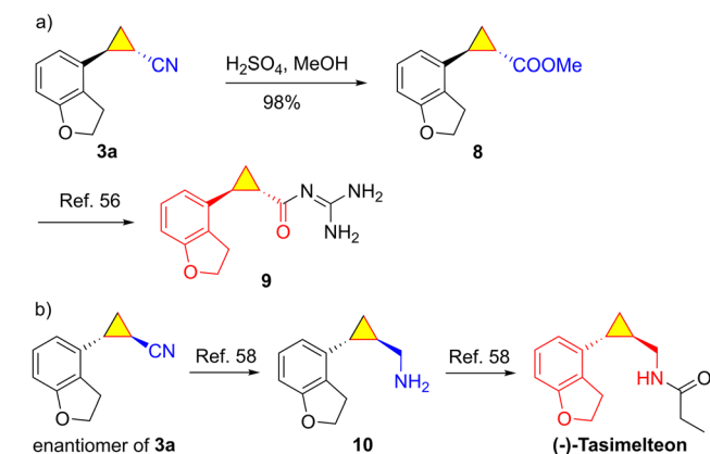
Scheme 5 (a) Preparation of 9 from 3a. (b) Preparation of (–)-Tasimelteon from the enantiomer of 3a.
