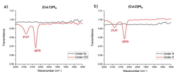
Fig. 2 IR spectra of (a) [\text{CuL1}]\text{PF}_6 under \text{N}_2 (grey) and CO (red) and (b) [\text{CuL2}]\text{PF}_6 under \text{N}_2 (grey) and CO (red).
