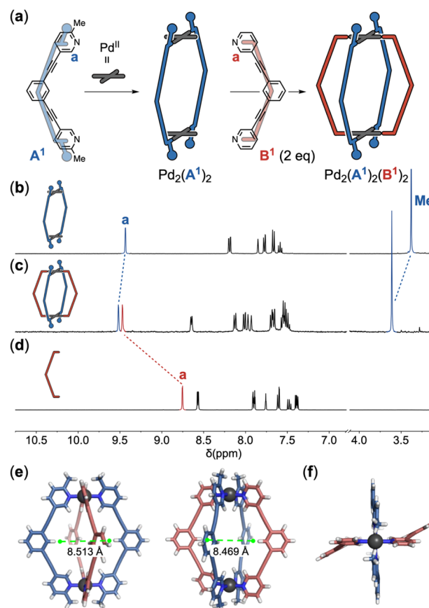
Fig. 2 Selective synthesis of the [\text{Pd}_2(\text{A}^1)_2(\text{B}^1)_2] cage. The reaction between ring assembly [\text{Pd}_2(\text{A}^1)_2] and 2 eq. of ligand \text{B}^1 yielded the cage [\text{Pd}_2(\text{A}^1)_2(\text{B}^1)_2] (a). Partial ^1\text{H} NMR spectra of ring assembly [\text{Pd}_2(\text{A}^1)_2] (b), cage [\text{Pd}_2(\text{A}^1)_2(\text{B}^1)_2] (c) and ligand \text{B}^1 (d) in acetonitrile. Full spectra can be found in the ESI.† The crystal structure of cage [\text{Pd}_2(\text{A}^1)_2(\text{B}^1)_2] in side view (e) and top view (f). Anions and solvent molecules are omitted for clarity.
