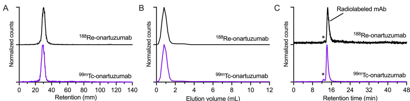
Fig. 5 Chromatographic data on the photoradiosynthesis of ^{99m}\text{Tc} -onartuzumab (purple traces) and ^{188}\text{Re} -onartuzumab (black traces) showing (A) iTLC chromatograms, (B) elution profiles recorded from manual elution of a PD-10 size-exclusion gel column, and (C) SEC-HPLC radio-chromatograms for the purified samples of each radiotracer. Note '*' indicates the elution of high molecular weight protein aggregates (dimers and higher order multimeric species). Equivalent chromatograms of the crude reaction mixtures are presented in ESI (Fig. S62–S64 and S65–S67†).
