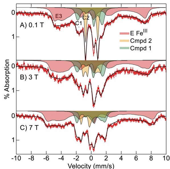
Fig. 5 Mössbauer spectra ((A–C) red vertical bars) of oxidized Ne bCcP at pH 8.6 reacted with 15 equivalents \text{H}_2\text{O}_2 recorded at 4 K in the magnetic fields listed. The black traces and filled areas are simulations (see text) for the parameters of Table 1.
