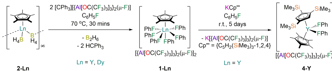
Fig. 1 Synthesis of 1-Ln (Ln = Y, Dy) by the separate reactions of parent 2-Ln with [\text{CPh}_3][\{\{\text{Al[OC(CF}_3\text{)}_3\}_3\}_2(\mu\text{-F)}\}] in fluorobenzene and synthesis of 4-Y by the reaction of 1-Y with \text{KCp}''' in fluorobenzene.
