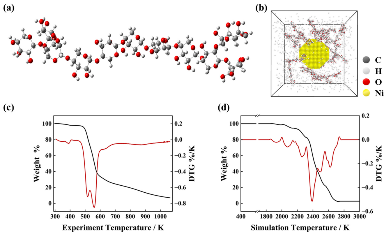
Fig. 1 (a) Constructed model of xylan, (b) initial simulation system of Ni-catalyzed hydropyrolysis of xylan, (c) experiment TGA result of xylan, and (d) simulation TGA result of xylan.
