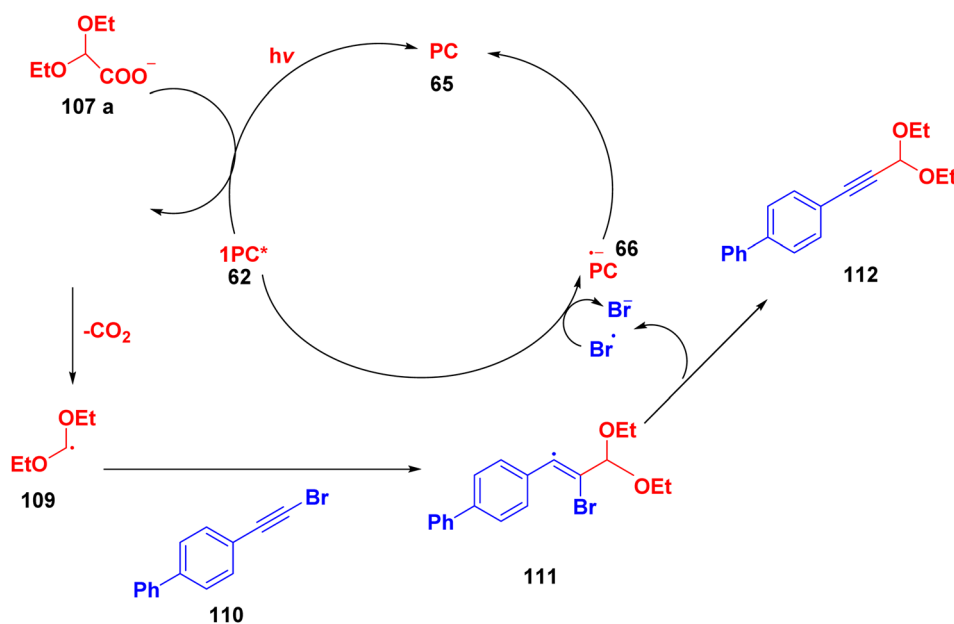
Fig. 59 Synthetic approach for the photocatalytic acetalation of alkynyl bromides. 240
