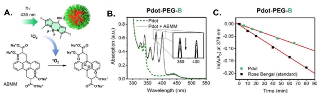
Fig. 41 Determination of the ^1\text{O}_2 quantum yield of Pdot-PEG-B: (A) diagram illustrating the photoexcitation of the Pdots and the subsequent degradation of an anthracene-based chemical acceptor (ABMM); (B) UV/vis spectra of a mixture of ABMM and Pdot-PEG-B in water after various irradiation times; (C) comparison of the first-order kinetics of ABMM degradation ( \lambda_{\text{max}} = 379 \text{ nm} ) in the presence of either Pdot-PEG-B or Rose Bengal. Reproduced from ref. 206, https://doi.org/10.1002/anie.202400712 , under the terms of the CC BY 4.0 license, https://creativecommons.org/licenses/by/4.0/ .
