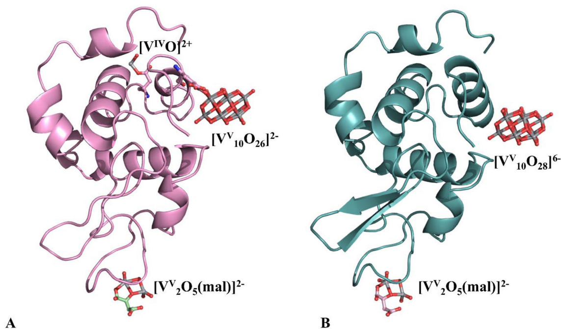
Fig. 6 Overall structures of V-HEWL adducts derived from two crystals of HEWL exposed to Cs 2 [V 2 O 4 (mal) 2 ]·2H 2 O for 7 days: (A) Structure A; (B) structure B. Vanadium atoms are in grey. Coordinates and structure factors were deposited in the PDB under the accession codes 9RBG, and 9RBT.
