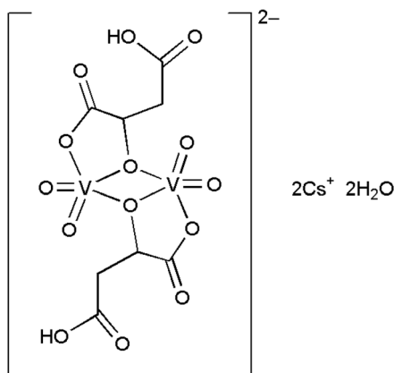
Fig. 1 Structure of Cs_2[V_2O_4(mal)_2] \cdot 2H_2O .
