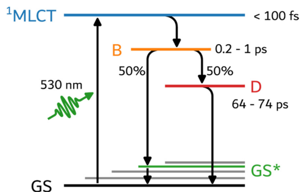
Fig. 8 Proposed relaxation scheme for the family of complexes. The ^1\text{MLCT} is populated and depleted within less than 100 fs. Its depopulation corresponds to the population of state B that decays over the ps timescale into a hot ground state \text{GS}^* and the long-living state D.
