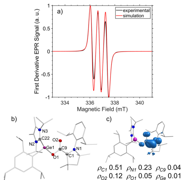
Fig. 3 (a) Experimental and simulated continuous-wave EPR spectra of a C 6 D 6 solution of 3 (simulation parameters: g = 2.0035 , A(^{14}\text{N}) = 6.0 G). (b) Molecular structure of NHC-germylene radical 3 in the solid state (co-crystallized solvent molecules and hydrogen atoms omitted for clarity, thermal ellipsoids at 50%). Selected bond lengths [Å] and angles [°]: Ge1–O1 1.9528(7), C9–O1 1.339(1), C9–O2 1.238(1), C1–N1 1.376(1), C1–C9 1.441(1), \angle(\text{Ge1}) 288.2(1). (c) Calculated Mulliken spin densities and spin density plot (contour value 0.0038).
