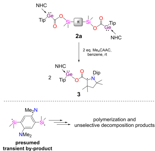
Scheme 4 Synthesis of paramagnetic NHC-germylene 3 (NHC = 1,3-diisopropylimidazol-4,5-dimethyl-2-ylidene, \text{CAAC}^{\text{Me}} = 1-(2,6-diisopropylphenyl)-3,3,5,5-tetramethyl-pyrrolidin-2-ylidene).
