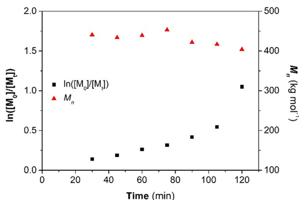
Fig. 2 \text{Fe}(\text{acac})_3 mediated conventional polymerization of MA at different polymerization time performed at \text{MA/Fe/Si-H} = 200/0.5/0.25 .
