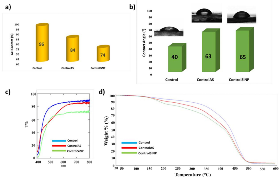
Fig. 18 The gel content values (a), water contact angle values (b), transmission spectra (c), and TGA thermograms (d) of the photoseets.
