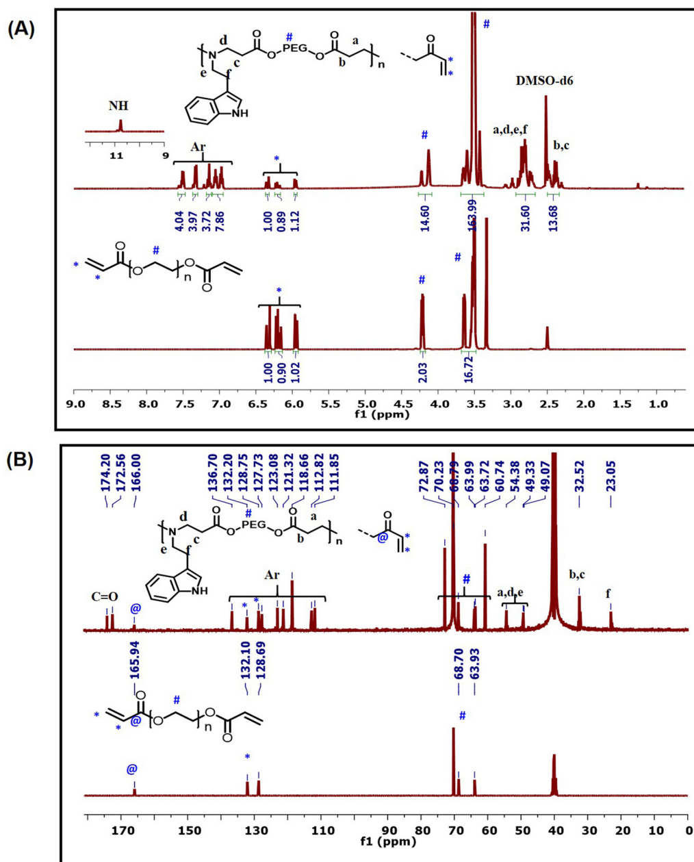
Fig. 2 (A) ^1\text{H} -NMR spectra and (B) ^{13}\text{C} -NMR spectra of InPEG 575 and PEG diacrylate (macromonomer).
