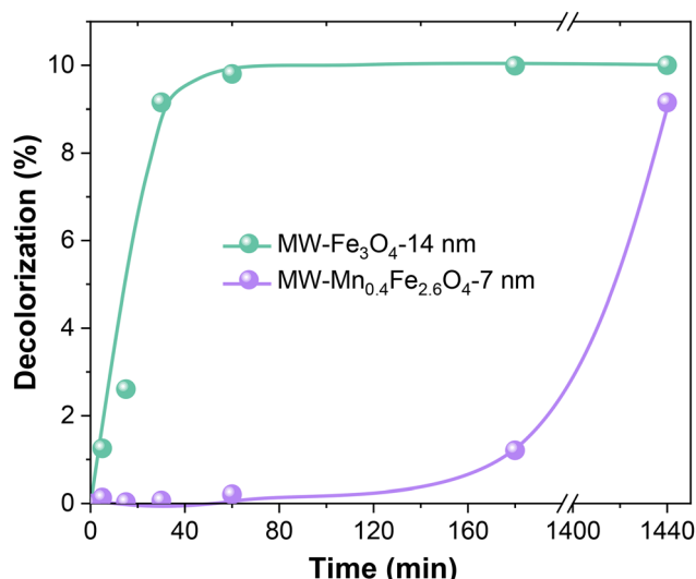
Fig. 8 Decolorization of methylene blue (MB, 100 ppm) using \text{MW-Fe}_3\text{O}_4 (green) and \text{MW-Mn}_{0.4}\text{Fe}_{2.6}\text{O}_4 (purple), [\text{H}_2\text{O}_2] = 0.03 M, [\text{NPs}] = 1 mg \text{mL}^{-1} at RT. Lines are included as guides to the eye. A blank experiment performed without catalyst exhibited 0% decolorization along the entire time range. An additional data point at 1440 min (24 h) was included for \text{Mn}_{0.4}\text{Fe}_{2.6}\text{O}_4 to capture the late-onset catalytic activity. The axis break reflects the gap between 180 and 1440 min. No further time points were added to avoid altering the system by replenishing \text{H}_2\text{O}_2 , ensuring all samples were compared under identical initial conditions.
