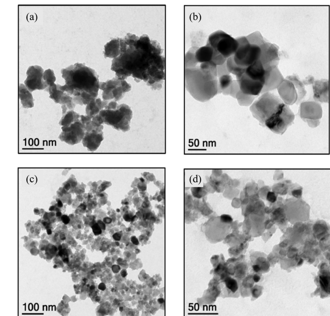
Fig. 14 HR-TEM images of biosynthesized NPs. (a) Native \text{TiO}_2 NPs; (b) anatase NPs; (c) anatase and rutile NPs mix; (d) rutile NPs. 183 Copyright © 2014 Elsevier Ltd. All rights reserved.
