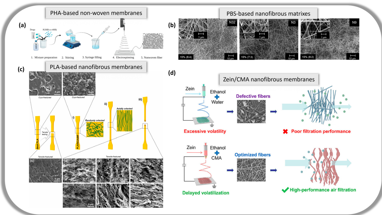
Fig. 2 (a) Schematic diagram of the process of obtaining PHA-based non-woven membranes loaded with antibiotic drugs via the electrospinning method. Reproduced from ref. 40 with permission from MDPI copyright 2023. (b) SEM images of electrospun biobased 15% (w/v) PBS fibrous matrices from \text{CHCl}_3 : \text{HCOOH} solutions. N32, N3 and N9 with solvent ratios of 6 : 4, 7 : 3 and 8 : 2 respectively. Reproduced from ref. 42 with permission from Elsevier Ltd. Copyright 2023. (c) SEM images of cryo-fractured cross-sections of (a) pristine PLA, (b) PLA–chitin reinforced nanofibers, and tensile-fractured cross-sections of (c) pristine PLA, (d–f) PLA–cellulose reinforced nanofibers, (g–i) PLA–chitin reinforced nanofibers. Reproduced from ref. 43 with permission from Elsevier Ltd. Copyright 2024. (d) Schematic illustration of the optimized electrospun zein/CMA nanofibers using the solution volatility optimization strategy compared to conventional pure zein nanofibers using ethanol and water for air filtration. Reproduced from ref. 44 with permission from American Chemical Society copyright 2023.
