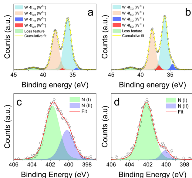
Fig. 2 (a and b) XPS spectra of the W 4f region of undoped (a) and MA-doped (b) \text{WO}_{3-x} NCs. (c and d) XPS spectra in the N 1s region for doped NCs before (c) and after (d) treatment with trifluoroacetic acid.
