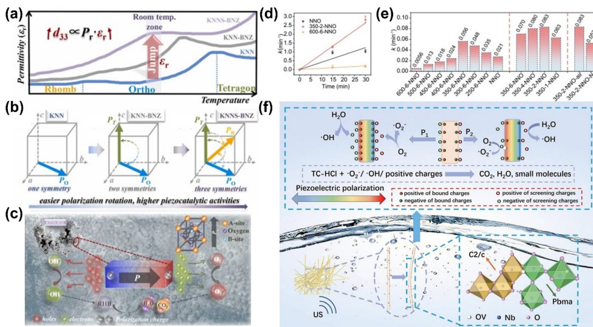
Fig. 5 (a and b) Schematic illustration of (a) temperature-dependent dielectric permittivity and (b) spontaneous polarization vector ( P_s ) of ( K_{0.5}Na_{0.5} )NbO 3 (KNN), ( K_{0.5}Na_{0.5} )NbO 3 -( Bi_{0.5}Na_{0.5} )ZrO 3 (KNN-BNZ), and Sb-doped ( K_{0.5}Na_{0.5} )NbO 3 -( Bi_{0.5}Na_{0.5} )ZrO 3 (KNNS-BNZ) samples. (c) Schematic illustration showing the generation of electrons and holes with their transfer for piezocatalysis. Reprinted with permission from ref. 93. Copyright 2022, Elsevier. (d) Pseudo-first-order kinetic fitting and (e) corresponding reaction rate constants of RC-HCl removal for NaNbO 3 nanowires annealed at different temperature, time, and atmospheres. (f) A proposed mechanism of piezocatalytic degradation of antibiotics by NaNbO 3 nanowires. Reprinted with permission from ref. 94. Copyright 2024, Elsevier.
