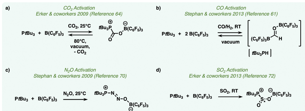
Fig. 6 Small molecule activation using \text{B}(\text{C}_6\text{F}_5)_3 FLPs. (a) \text{CO}_2 activation & capture using \text{PtBu}_3 and \text{B}(\text{C}_6\text{F}_5)_3 at 25 °C results in a \text{PtBu}_3\text{CO}_2\text{B}(\text{C}_6\text{F}_5)_3 complex, where \text{CO}_2 can be liberated at 80 °C under vacuum. 64 (b) \text{CO} activation & capture using \text{PtBu}_3 and 2[\text{B}(\text{C}_6\text{F}_5)_3] at room temperature in the presence of \text{H}_2 to form a formyl borate derivative, which can be reversed to release \text{CO} upon placing under vacuum. 61 (c) \text{PtBu}_3 , \text{B}(\text{C}_6\text{F}_5)_3 , & \text{N}_2\text{O} form a bridged \text{B}(\text{C}_6\text{F}_5)_3\text{--N}_2\text{O--PtBu}_3 species in a trans configuration upon combining the reagents and heating at 25 °C. 70 (d) \text{PtBu}_3 , \text{B}(\text{C}_6\text{F}_5)_3 , & \text{SO}_2 react at room temperature to form a bridged zwitterionic \text{B}^+(\text{C}_6\text{F}_5)_3\text{--SO}_2\text{--P}^+\text{tBu}_3 adduct. 72
