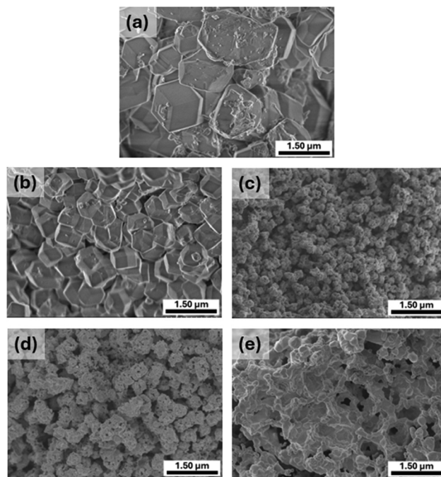
Fig. 4 SEM images of (a) Fe-ZIF-8, (b) Fe-ZIF-8 300, (c) Fe-ZIF-8 500, (d) Fe-ZIF-8 700, and (e) Fe-ZIF-8 900 at 20 000 \times magnification.
