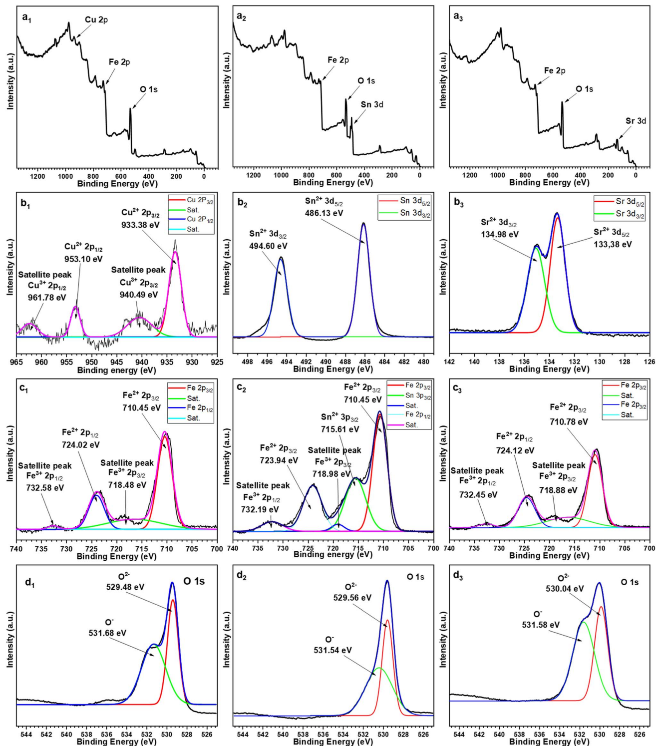
Fig. 5 XPS survey (a 1 –a 3 ), high-resolution M (M = Cu 2p, Sr 3d, and Sn 3d) (b 1 –b 3 ), Fe 2p (c 1 –c 3 ) and O 1s spectra (d 1 –d 3 ) of CuFe 12 O 19 , SnFe 12 O 19 , and SrFe 12 O 19 , respectively.
