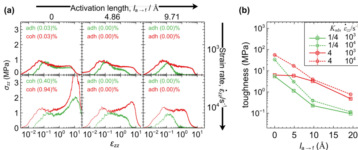
Fig. 14 (a) Stress-strain curves and (b) toughness as a function of the activation length l_{a \rightarrow f} , elongation rate \dot{\epsilon}_{zz} = 10^3 s ^{-1} (solid line, squares), 10^4 s ^{-1} (dashed line, circles) and equilibrium adsorption constant K'_{ads} = k'_{f \rightarrow a}/k'_{a \rightarrow f} = 1/4 (green) and 4 (red). In all cases k'_{a \rightarrow f} = 10^2 s ^{-1} . The legends in (a) denote the failure mode (adhesive or cohesive) and the percentage of ruptured strands for each case.
