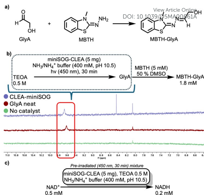
Figure 5: Photochemical generation of glycolaldehyde (GlyA) and NADH using miniSOG-CLEA. a) GlyA derivatisation with 3-methyl-2-benzothiazolinone hydrazone (MBTH) to give the UV-detectable adduct MBTH-GlyA. b) GlyA formation: irradiation of miniSOG-CLEA (5 mg) in 0.5 M TEOA / 400 mM \text{NH}_3/\text{NH}_4^+ buffer (pH 10.5) for 30 min (450 nm) affords 1.8 mM GlyA, quantified as MBTH-GlyA. No GlyA is detected in dark or “no-CLEA” controls. ^1\text{H} -NMR spectra of highlighted reaction products. Peak at \approx 9.5 can be attributed to miniSOG degradation. c) The pre-irradiated mixture (pre- \text{NAD}^+ addition) reduces \text{NAD}^+ (0.5 mM) to enzymatically active NADH (0.2 mM) within 1 h in the dark, confirming GlyA-mediated cofactor regeneration.
