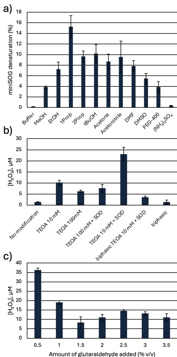
Figure 2: a) Precipitant screen. b) Reaction additive screen. c) Glutaraldehyde dose optimisation. All data represent mean \pm SD ( n = 3 ). H 2 O 2 quantification determined by HRP/ABTS assay using a calibration curve (Fig. S6).
