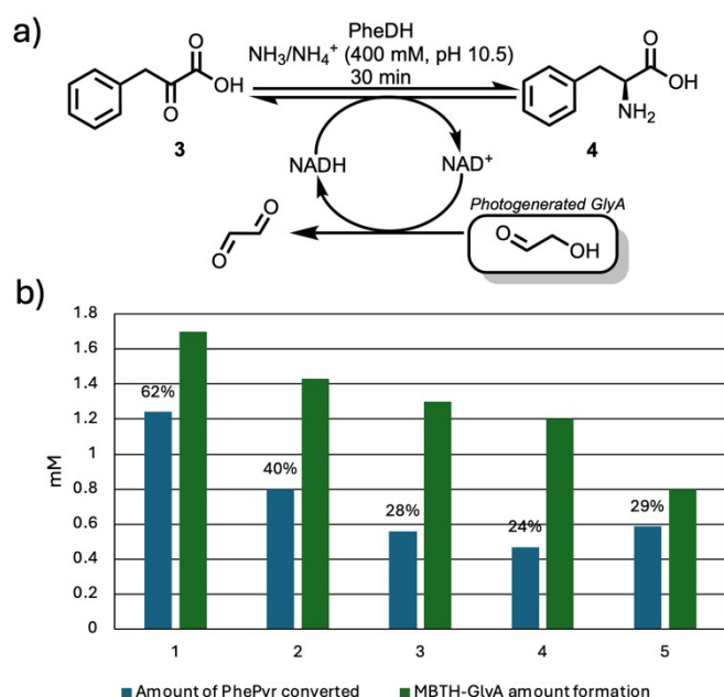
Figure 6: Coupling photogenerated glycolaldehyde to PheDH-catalysed reductive amination. a) Reaction scheme. b) Recycling study (five 30-min irradiation cycles; 5 mg CLEA, 0.5 M TEOA, 0.2 mM NAD + , in 1 mL). Blue bars: PhePyr converted (%) Green bars: GlyA formed (mM, quantified as MBTH adduct). Product formation parallels GlyA availability. No product was detected in “no-light” or “no-CLEA” controls.
