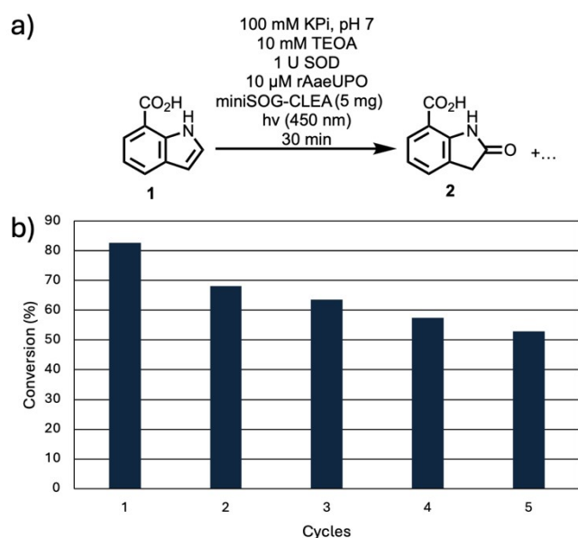
Figure 4: a) Reaction scheme and conditions for the blue-light mediated oxidation of 1 (1 mM) to oxindole 2 using rAaeUPO and in-situ produced H 2 O 2 from miniSOG-CLEA. b) Recyclability test of the miniSOG-CLEA photocatalyst.
