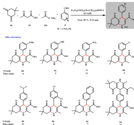
Scheme 46 Catalytic synthesis of hexahydroquinoline derivatives using an Fe 3 O 4 @SiO 2 @Si-(CH 2 )@HMAT@Cu nanocomposite (Salem et al. ).
