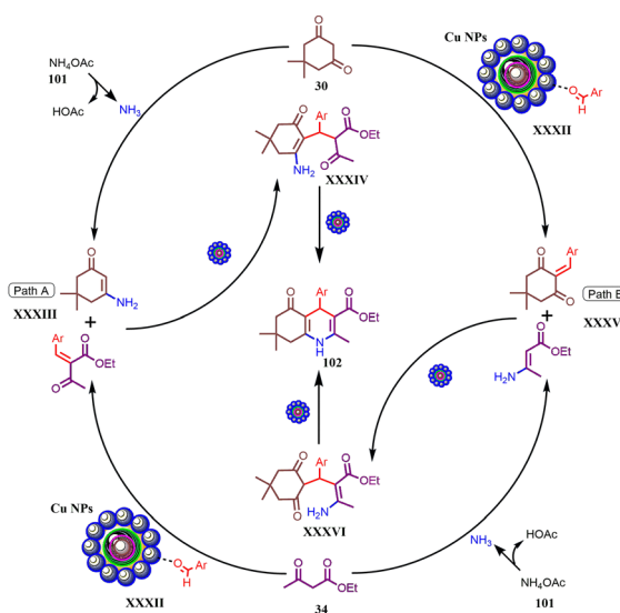
Fig. 11 Plausible mechanism for synthesis of hexahydroquinoline derivatives using an Fe 3 O 4 @SiO 2 @Si-(CH 2 )@HMAT@Cu nanocomposite (Salem et al. ).
