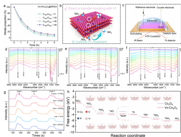
Fig. 4 (a) Time profile of \text{NO}_3^- removal curves with or without the addition of TBA. (b) Mechanism schematic diagram of the \text{eNO}_3^- -RR on \text{Vo-HCo}_3\text{O}_4@\text{SRGA} . (c) Schematic illustration of the in situ electrochemical FT-IR. In situ FT-IR spectra of (d) \text{H-Co}_3\text{O}_4 , (e) \text{H-Co}_3\text{O}_4@\text{SRGA} , and (f) \text{Vo-HCo}_3\text{O}_4@\text{SRGA} during the \text{eNO}_3^- -RR. (g) Online DEMS spectra of \text{Vo-HCo}_3\text{O}_4@\text{SRGA} . (h) Free-energy diagrams and corresponding reaction intermediates of the \text{eNO}_3^- -RR of \text{Co}_3\text{O}_4 and \text{Vo-Co}_3\text{O}_4 .
